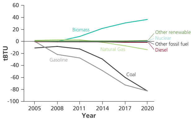
Figure 5.6 Modeled changes in fuel use under the “GGRA Case” relative to the reference case through 2020.
