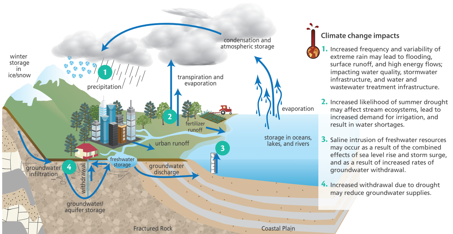
Figure 8.5 Climate change impacts on water resources.
