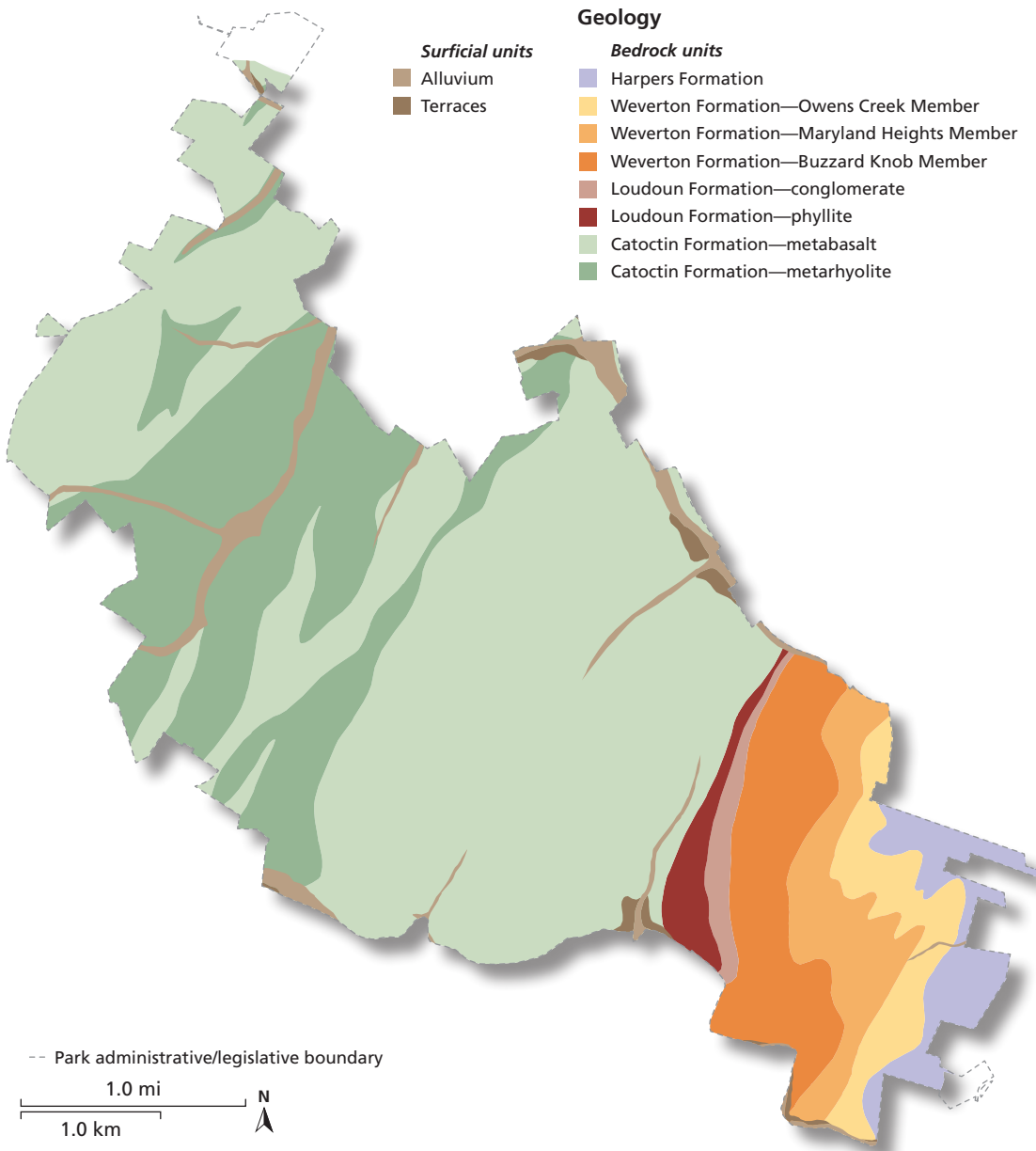
Figure 2.8. Geology of CATO (Thorneberry–Ehrlich 2009).
